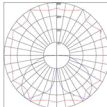
Maximum Candela = 603.85 Located At Horizontal Angle = 0°, Vertical Angle = 35° # 1 - Vertical Plane Through Horizontal Angles (0° - 240°) (Through Max. Cd.) # 2 - Horizontal Cone Through Vertical Angle (35°) (Through Max. Cd.)
