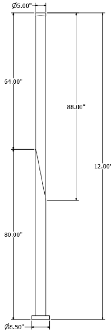
Diagonal Cut Column
