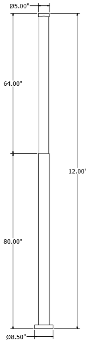
Horizontal Cut Column
